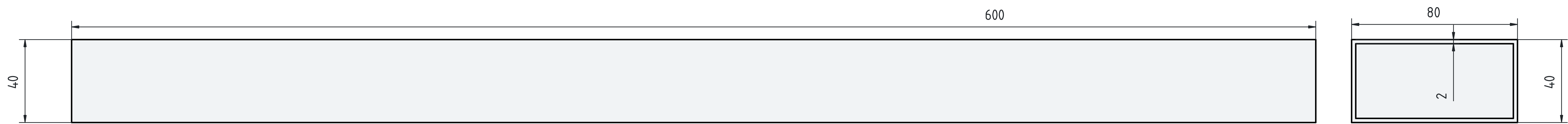
Besi hollow galvanis 80x40mm tebal 2mm
